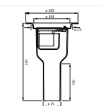
SIPHON STAINLESS STEEL 40* ref. 1416 007 outflow 0.25L/s
