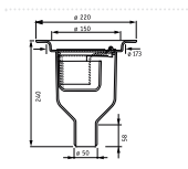
SIPHON PURUS DUSCH BRUNN 50 ref. 1416 001 outflow 2L/s
